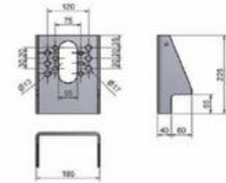
SUPPORT DE VASE STANDARD BRACKET FOR BOOSTER GRUNDPLATTE
